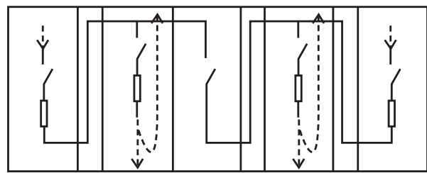
Line-up (main-tie-main)
